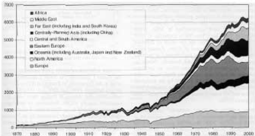
Greenhouse gas emissions from fossil fuels, in million tons carbon equivalent
